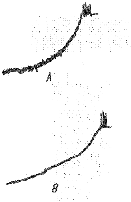
Fig. 1. ADP-induced platelet aggregation in vitro and the influence of 5% solution of Cernitin T60 [B] in comparison with control [A].
